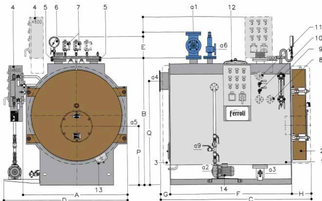
Key - 1 Boiler 2 Door 3 Smokebox 4 Electrical panel 5 Level pipe 6 Pressure gauge 7 Pressure switches 8 Surface drain pipe (optional) 9 Level gauge 10 Level test cocks 11 Level indicator (optional) 12 Manhole 13 Opening 14 Supply pump a1 Steam outlet a2 Pump inlet a3 Boiler drain a4 Flue outlet a5 Burner attachment fitting a6 Safety discharge a9 Auxiliary inlet
